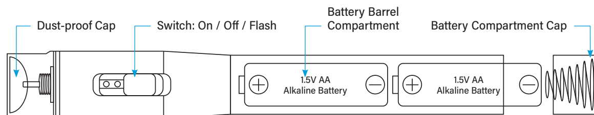
(Schematic Drawing)
